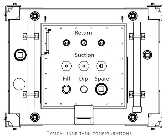
TYPICAL INNE TANK CONFIGURATIONS
